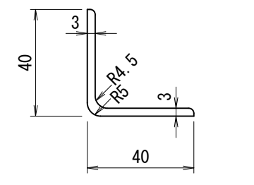
胴縁断面図 (R付L40x40x3) (S=1/2)
