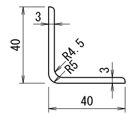
隅縁断面図 (R付L40x40x3) (S=1/2)
