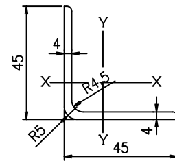
網締断面図 (R付L45x45x4) (S=1/1)
